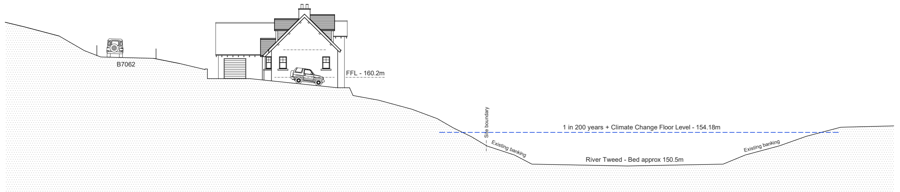
Cross Section through Application Site taken on East Gable of house looking West
